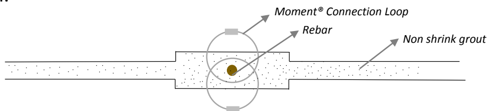
Drawing showing the top view of the connection in between the precast elements
